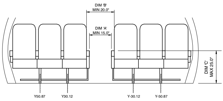
DETAIL E AISLE WIDTH - TYPICAL, ALL ROWS NTS
