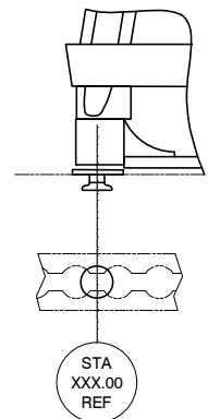
2 DETAIL D SEAT FWD STUD LOCATION NTS
